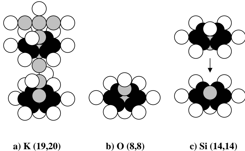
Fig. 2. Diagrams of the atomic nuclei of: a) potassium, b) oxygen, c) silicon
