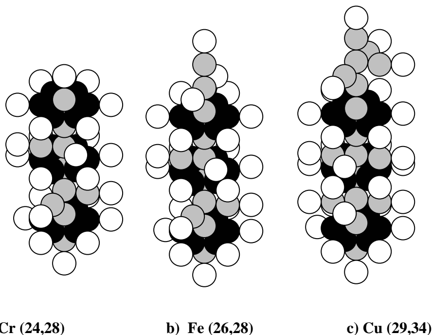
Fig. 1. Diagrams of the atomic nuclei of: a) chromium, b) iron, c) copper
