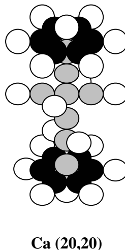
Fig. 4. Diagram of the nucleus of the calcium atom
