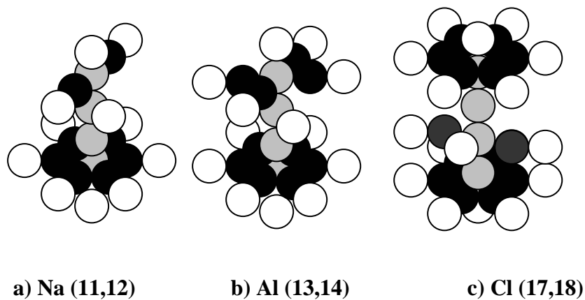
Fig. 3. Diagrams of the atomic nuclei of: a) sodium, b) aluminium, c) chlorine
